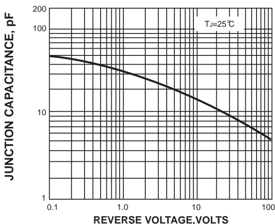
FIG. 5-TYPICAL JUNCTION CAPACITANCE
