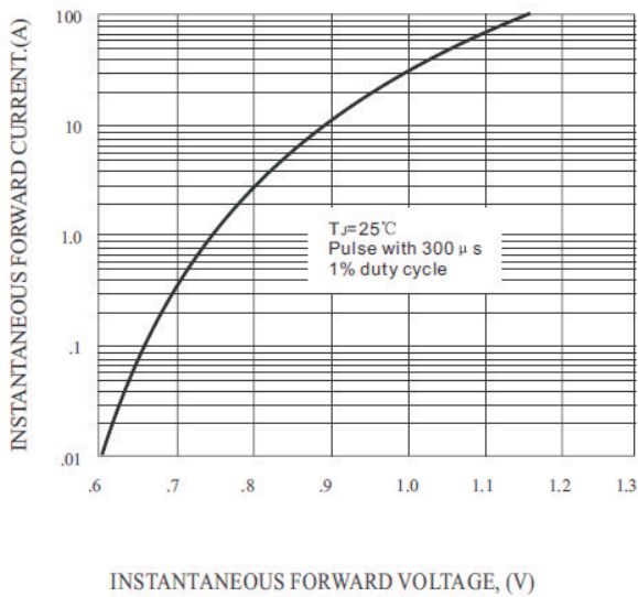
FIG.3-TYPICAL FORWARD CHARACTERISTICS
